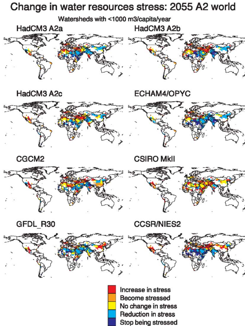
Fig. 6. Effect of climate change on water-stressed watersheds, 2055: A2 scenarios.
