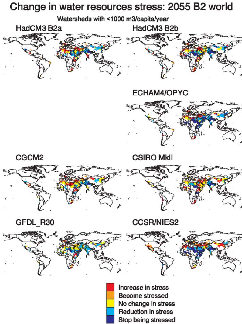
Fig. 7. Effect of climate change on water-stressed watersheds, 2055: B2 scenarios.
